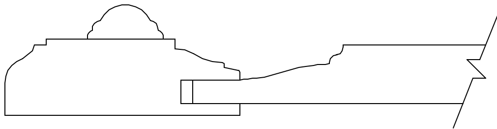
WMDRP-61 RAISED PANEL (With or without Moulding) MIN. 6 7/8"W X 6 7/8"H
