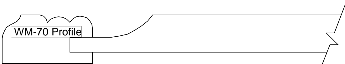
WMDRP-70 RAISED PANEL MIN. 5 3/4"W X 5 3/4"H
