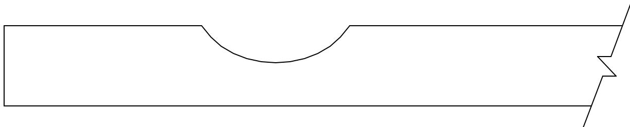
ROUTED PANEL 1 PASS ROUT (MDF ROUTED (WIDE ROUT) ONLY)
